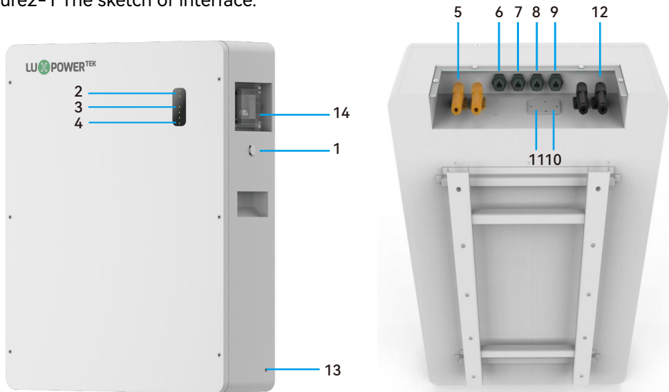
Figure2-1 The sketch of interface.
