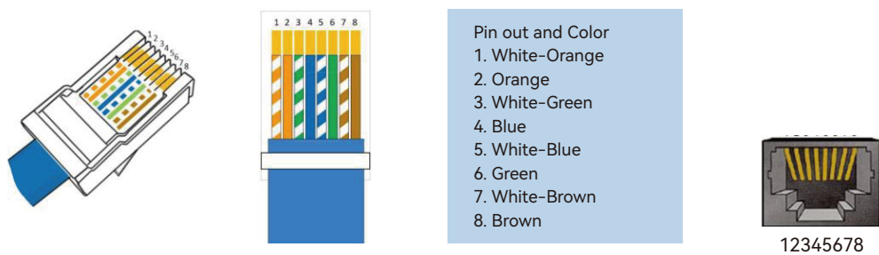
Figure 2-2 CAN, RS485, OUT, IN interface definition
